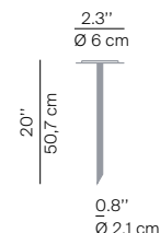
D13G.air/3 stake for inserting into the soil
